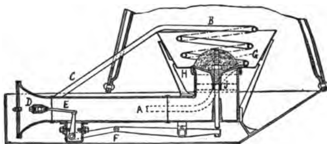
FIG. 204.—The Clarkson-Capel Kerosene Vapor Burner. A is the oil feed tube; B , the vaporizing coil; C , the pipe for gas for regulating valve; D ; E , the spindle of the needle valve; F , the operating lever of the valve; G , the gland of the burner; H , the variable opening for the flame.
